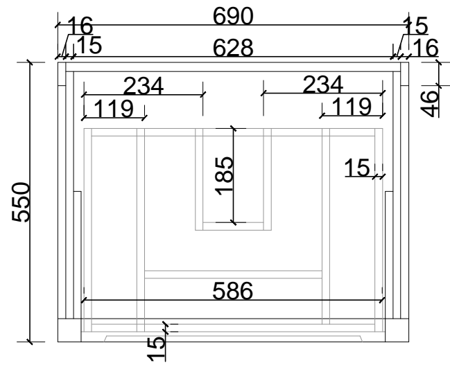
Plane View
